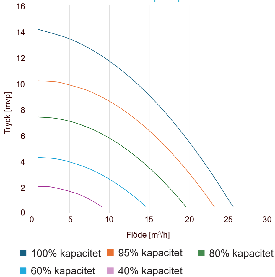
MiniVISE vs pumpkurva
