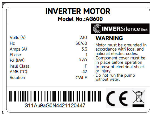
Picture 4. Rating plate - pump motor.
