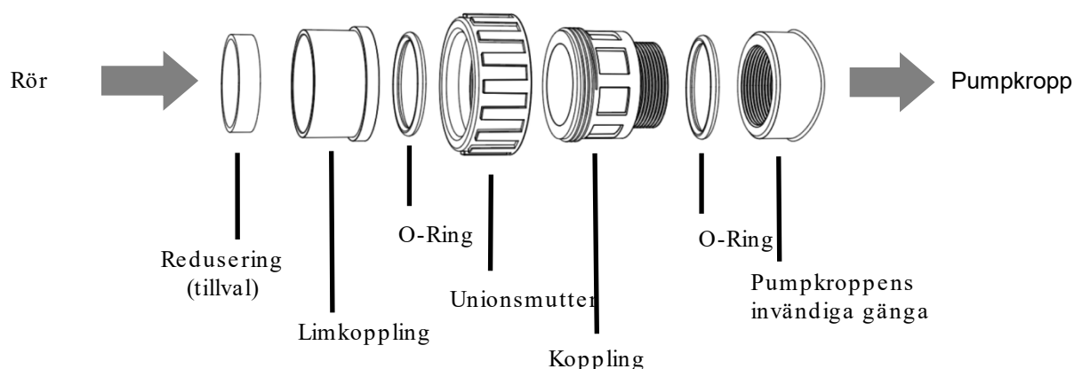
Figur 3 – Union Kit
