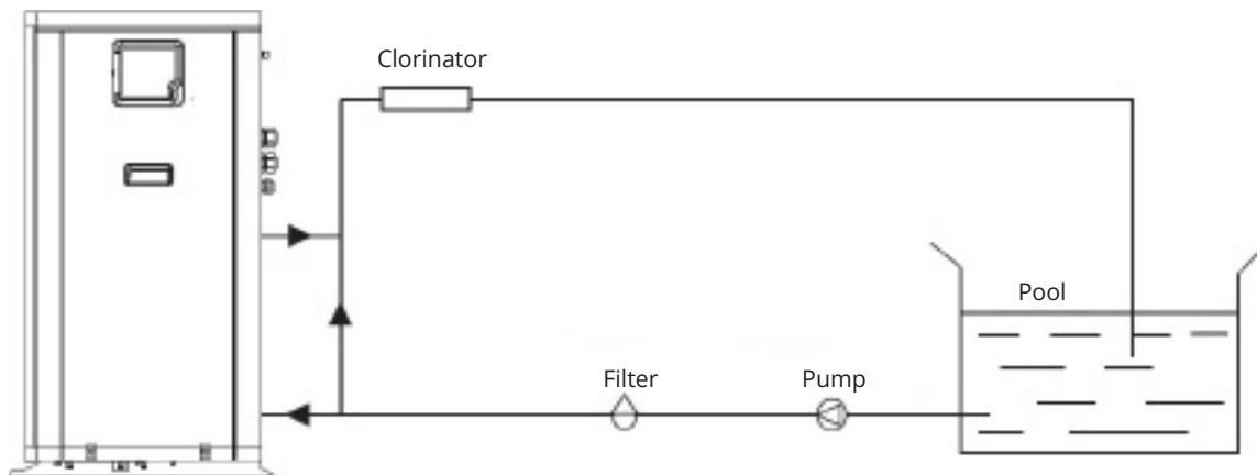
Installation schematic
